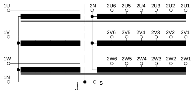
Principle diagram of the transformer T90
