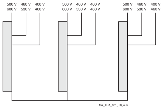
Connection example for ErP compliant fan for 500 V AC
