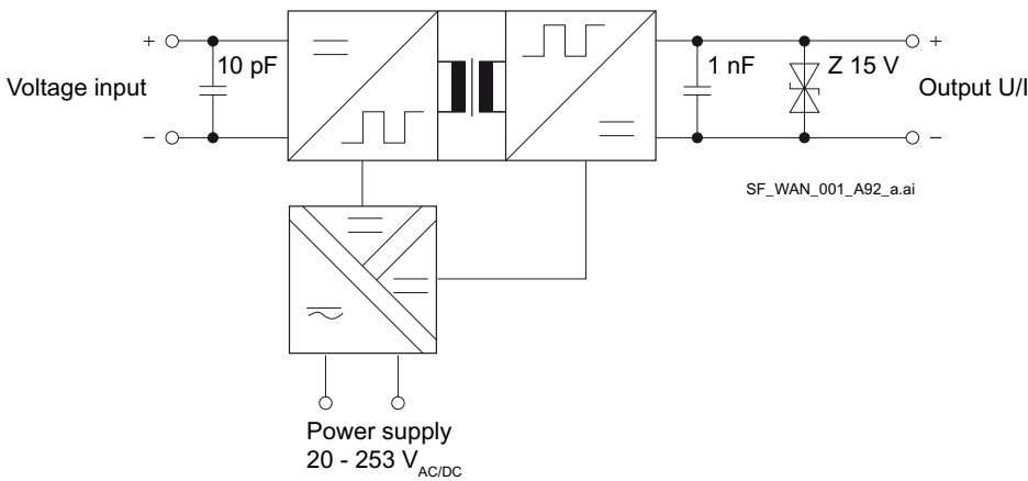
Principle circuit diagram of the DC-DC transducer A92 (1)
