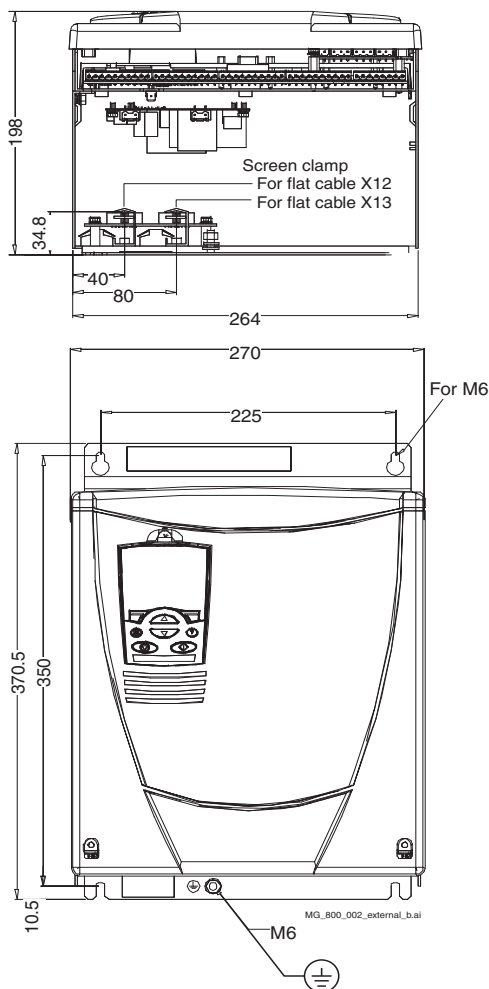
Control unit
