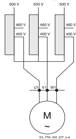
Connection example for ErP compliant fan for 500 V AC
