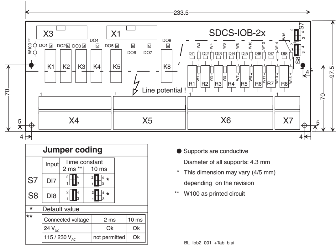
Layout and jumper settings of the SDCS-IOB-2x
