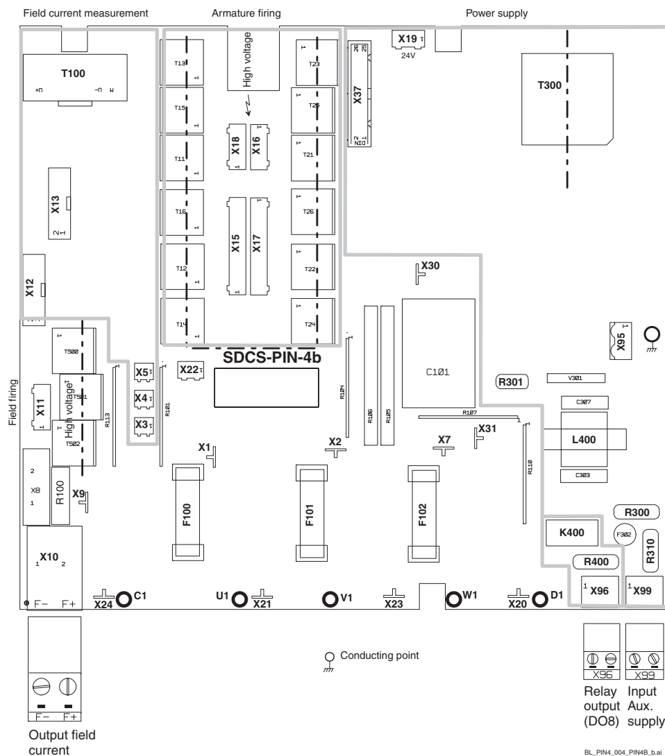
Layout SDCS-PIN-4b
