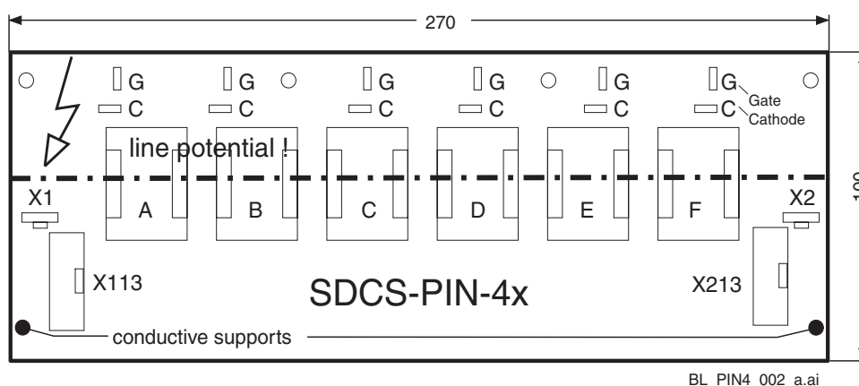
Layout of the SDCS-PIN-46 / SDCS-PIN-48
