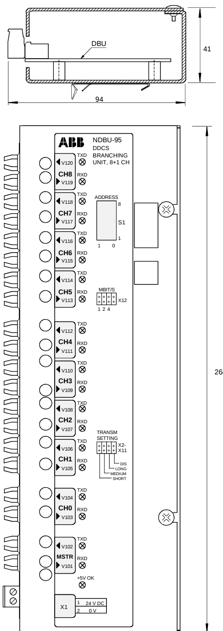
Layout of the NDBU-95
