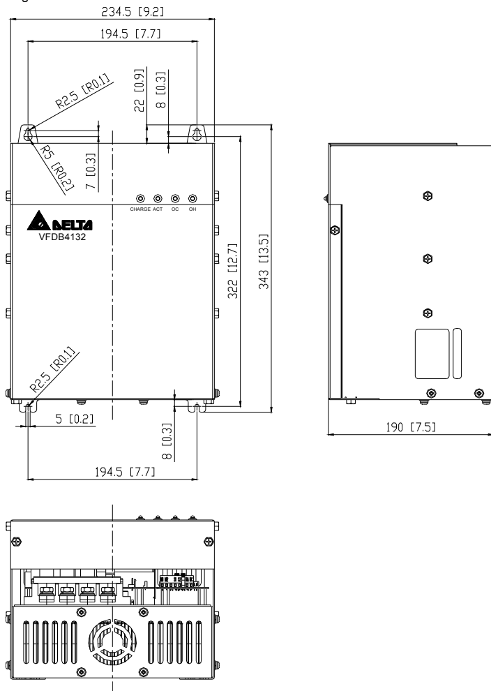
Figure 2: VFDB4132
