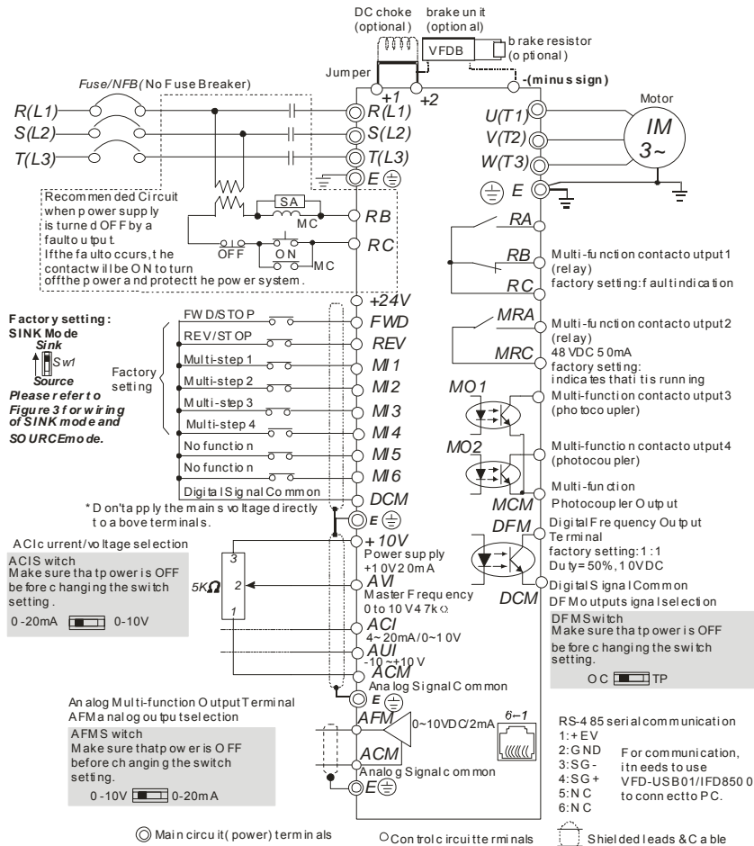
Figure 2 for models of VFD-VE Series (15HP/11kW and above) VFD150V23A/43A-2, VFD185V23A/43A-2, VFD220V23A/43A-2, VFD300V43A-2, VFD370V43A-2, VFD450V43A-2, VFD300V23A-2, VFD370V23A-2, VFD550V43C-2, VFD750V43C-2
