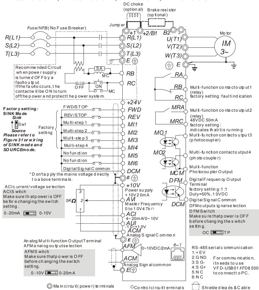
Figure 1 for models of VFD-VE Series (10 HP/7.5kW and below) VFD007V23A/43A-2, VFD015V23A/43A-2, VFD022V23A/43A-2, VFD037V23A/43A-2, VFD055V23A/43A-2, VFD075V23A/43A-2, VFD110V43B-2, VFD110V23A/43A-2
