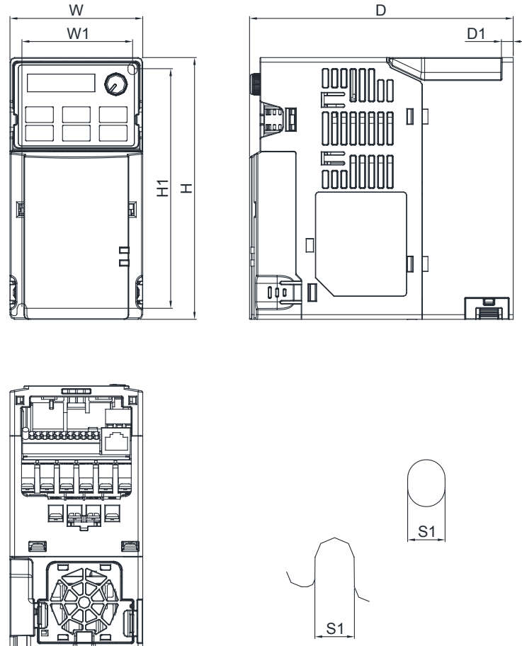
Mounting hole
